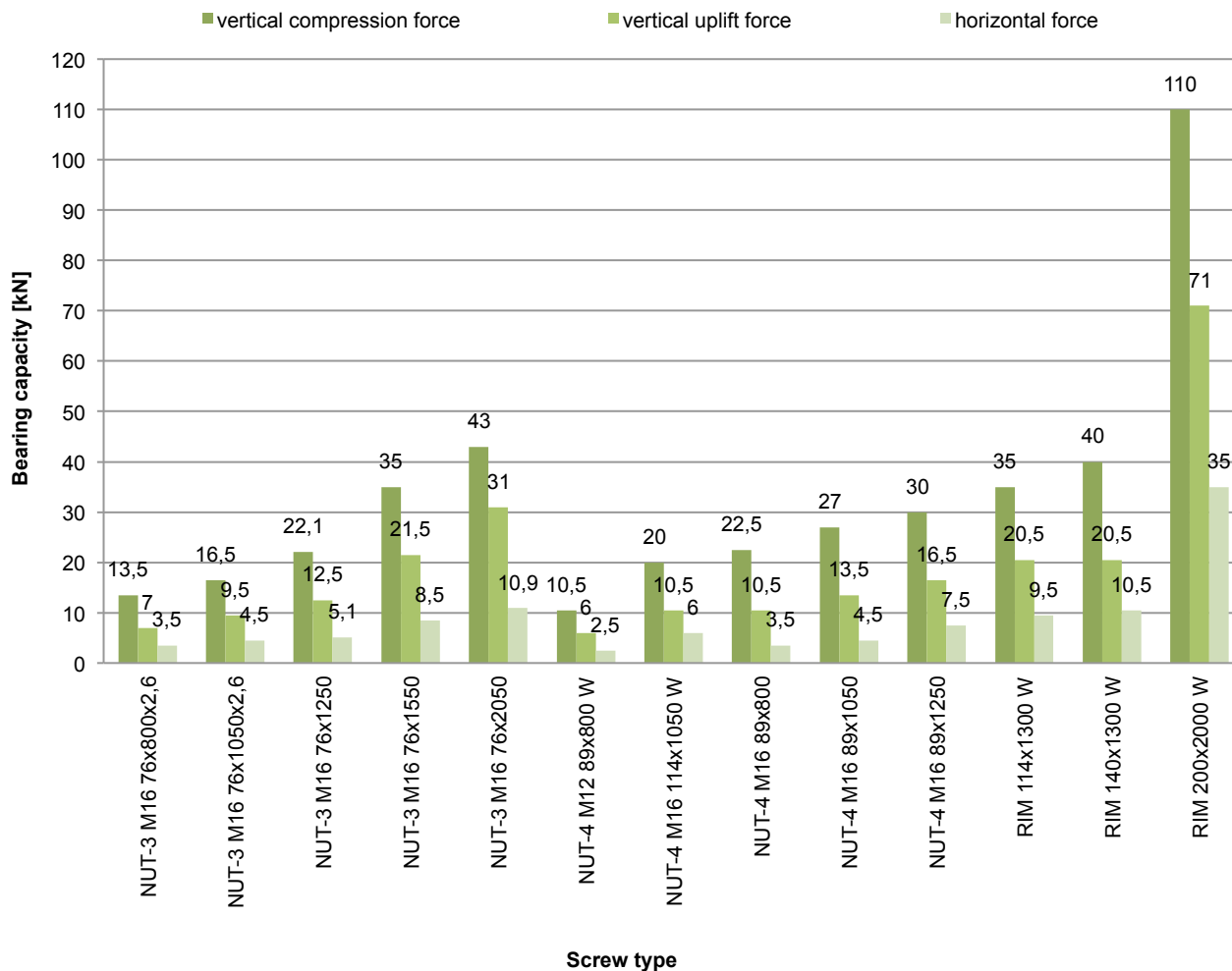
LOAD CHART
